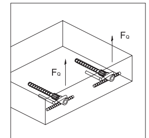
Shear Lift
